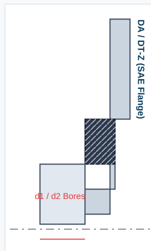
Figure 1: Sectional technical architecture showing direct engine flywheel mounting profile and concentric dual-stage dampening core.
